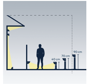
RAZE Wall-mounted
