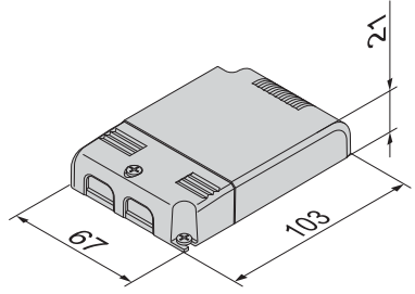
96107649 MAXI JOLLY 1-10V/15W
